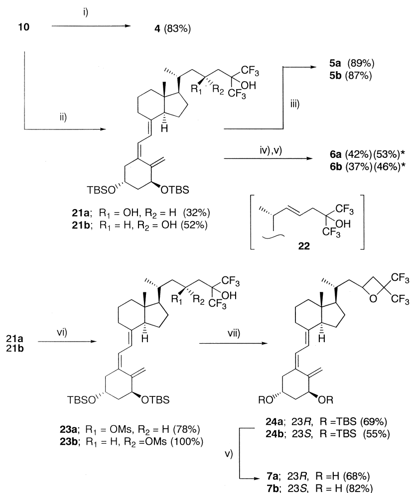
Scheme 3. (i) TsOH, MeOH, rt, 2 h; (ii) NaBH 4 , THF-MeOH, −10 °C, 10 min; (iii) MsOH, MeOH, rt, 1 h; (iv) DAST, CH 2 Cl 2 , −50 °C→rt, 1 h; (v) TBAF-THF, rt, overnight; (vi) MsCl, pyridine, 0 °C, 1 h; (vii) 5% KOH-MeOH; rt, 10 min. *Considering the recovery of starting material.
