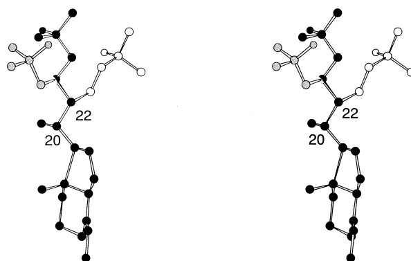
Figure 2. Superposition of three families of conformers of 5a , 5b , 6a and 6b at 0–6 kJ/mol (stereoview) as their deprotonated and defluorinated forms. The substituents at C-23 were omitted to see the orientation of side chains clearly.
