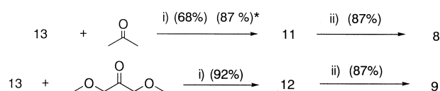
Scheme 4. (i) LiN(TMS) 2 , THF, −78 °C, (ii) MsOH, MeOH, rt, 1 h *Considering the recovery of 13 .
