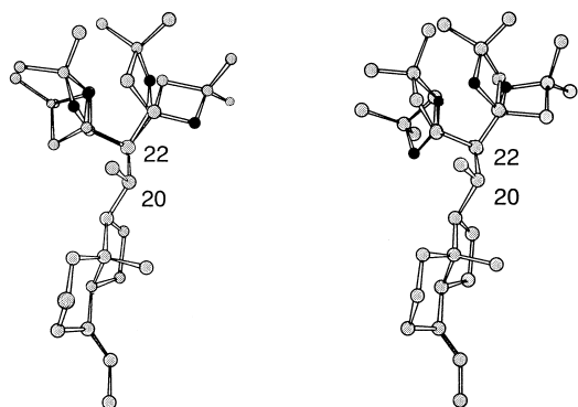
Figure 3. Superposition of four families of conformers of two oxetane compound ( 7a ; left, 7b ; right) at 0–8 kJ/mol as their deprotonated and defluorinated forms.
